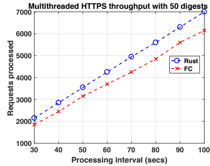
Figure 4: Throughput of an openssl HTTP in 30–100 seconds. Each request has 50 calls to ring’s digest. In the FC-enabled server, each digest iteration creates and releases a secure compartment.
