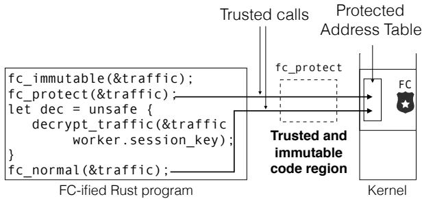
Figure 2: The trusted region is an address (in the code of FC's user space library) to which calls from mprotect must return to, which is ensured by FC's kernel module.
